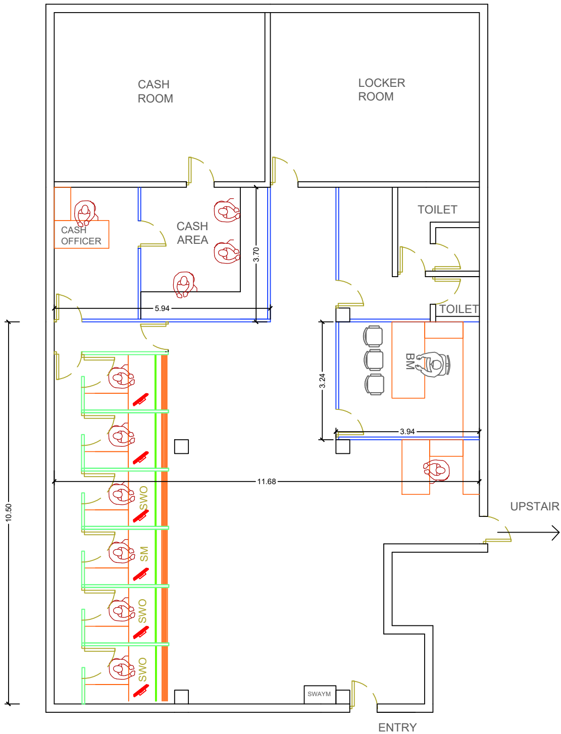
INTERIOR LAYOUT FOR VIRAR BRANCH(GR. FLOOR) - THANE
